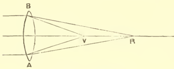
Chromatic Aberration.
